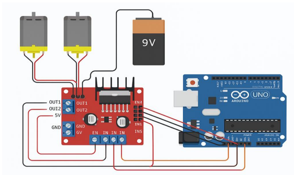
Figure 10: The Arduino Project connected
