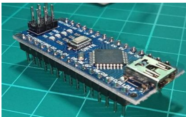
Figure 5: ARDUINO NANO
