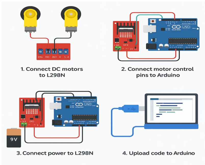
Figure 9: diagramatic steps of connecting components
