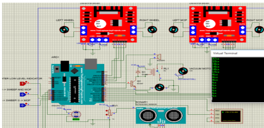
Figure 8: Proteus Simulation mode Agbeyangi et al, 2020
