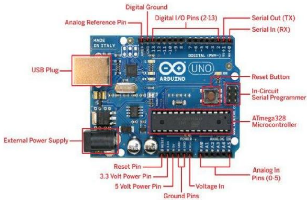
Figure 1: Arduino Pin configuration parts
